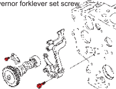
Fuel camshaft set screw &amp; Governor forklever set screw
