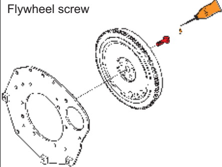
Flywheel screw
